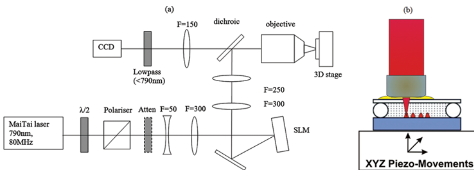
Figure 6. (a) Schematic diagram of the experimental setup for the fabrication process. (b) The sample is mounted on a xyz-piezoelectric translation stage and can be scanned under the high aperture objective used to focus the beam. (Figure appears in color online.)
