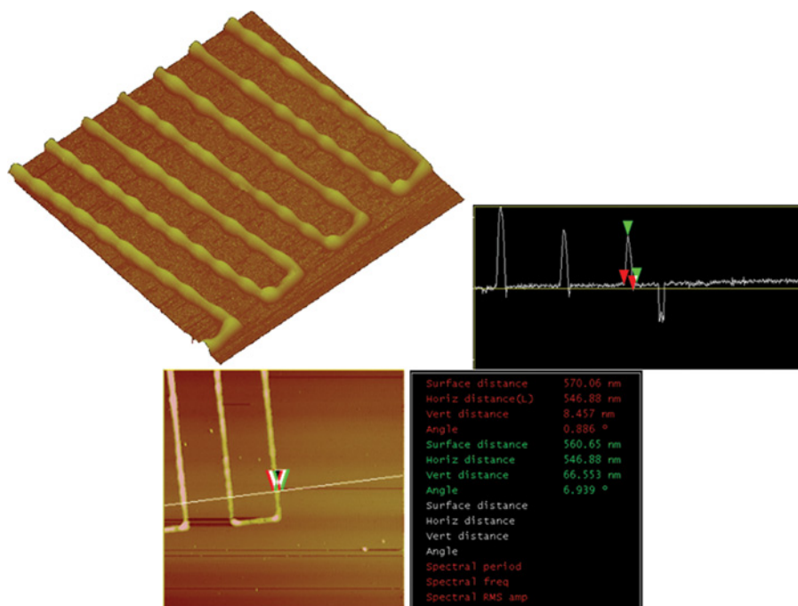
Figure 7. AFM measurements performed on the periodic surface structures. The lines are 2\text{ }\mu\text{m} spaced and their height is 0.1\text{ }\mu\text{m} . (Figure appears in color online.)
