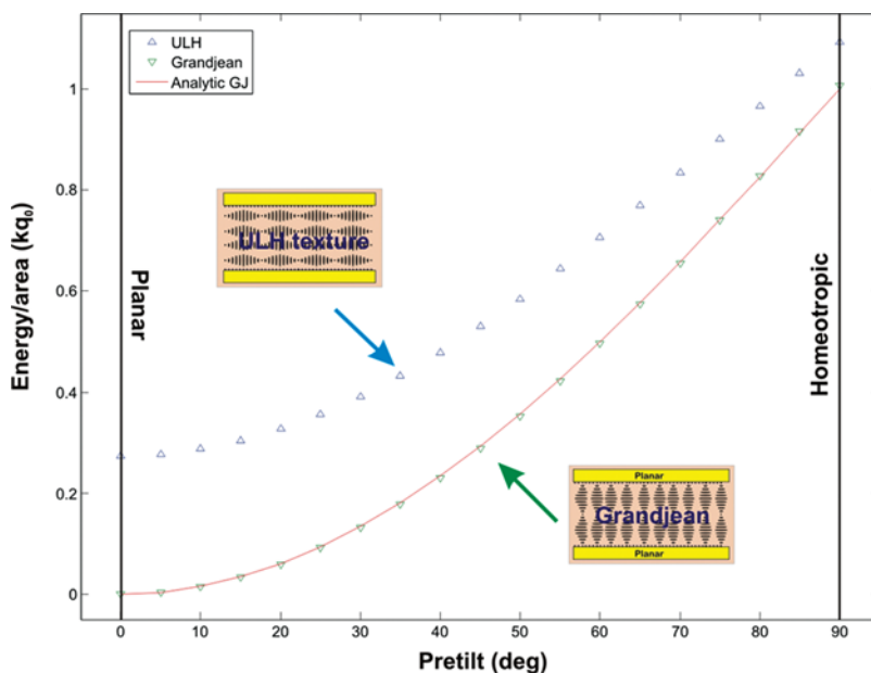
Figure 3. Elastic free energy of the interface region between a UAS and a bulk ULH ( \triangle ) and between a UAS and a Grandjean ( \nabla ) as a function of the pretilt \theta evaluated by finite difference numerical simulation. The continuous line is the analytic solution corresponding to the interface for the Grandjean texture. (Figure appears in color online.)
