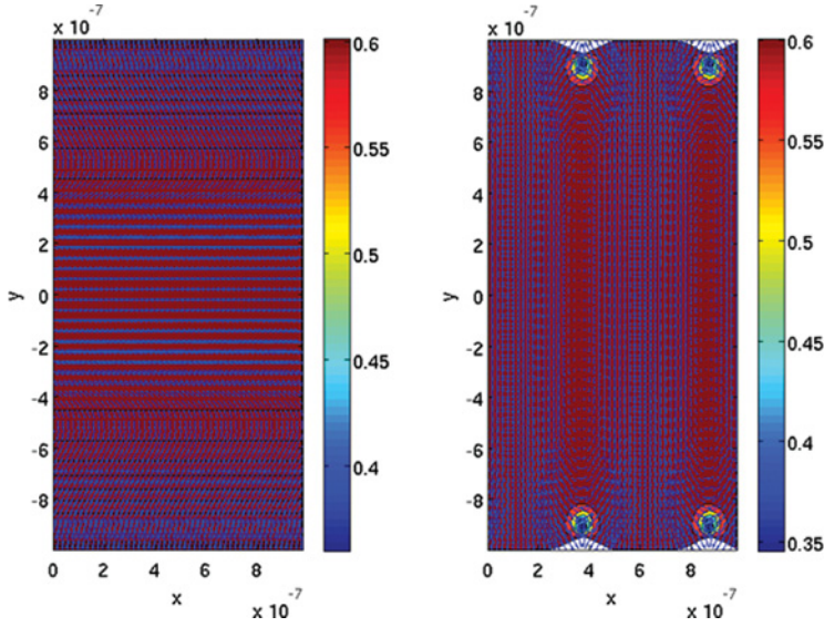
Figure 9. (a) The psuedo-Grandjean texture is the lower energy state for flat substrates. The blue arrows show the x and y components of the director while the background colour indicates the principal order parameter S according to colour bar shown. (b) With surface relief the ULH structure is the more stable. We clearly see the presence of strength -\frac{1}{2} defects. (Figure appears in color online.)
